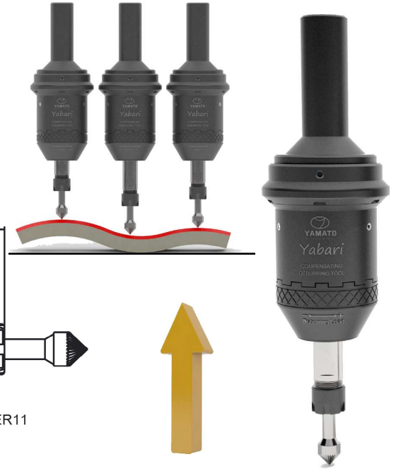
10mm AXIAL DEFLECTION PUSHING
